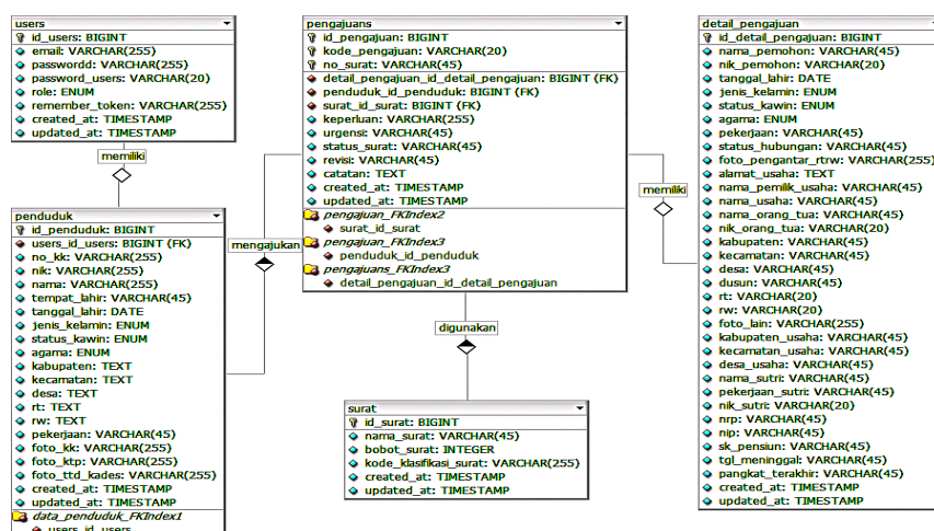
Gambar 8. Physical Database Design
