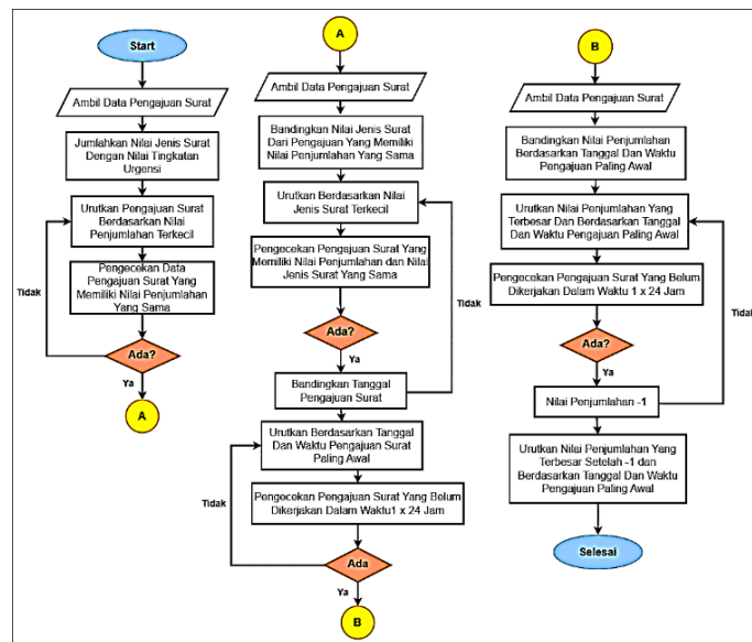
Gambar 1. Flowchart Penerapan Algoritma Shortest Job First
