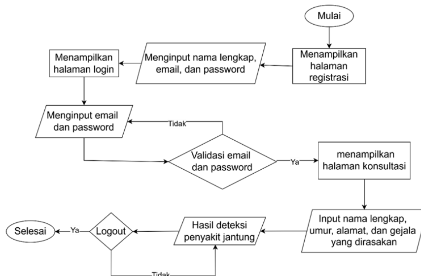
Gambar 3. Tampilan Flowchart
